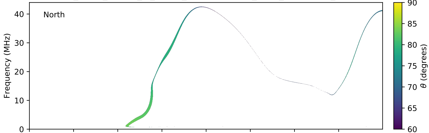
expres_earth_jupiter_io_jrm09_lossc-wid1deg_3kev_20061212_v01.cdf
