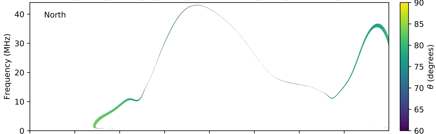
expres_earth_jupiter_io_jrm09_lossc-wid1deg_3kev_20061205_v01.cdf
