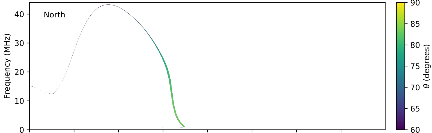
expres_earth_jupiter_io_jrm09_lossc-wid1deg_3kev_20061202_v01.cdf
