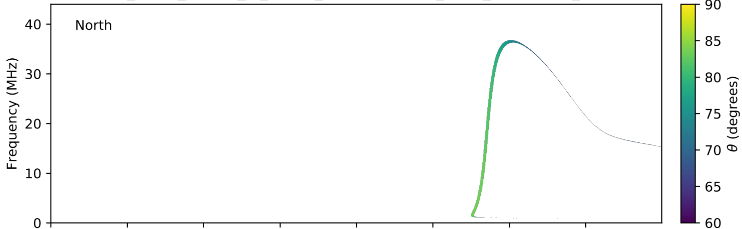
expres_earth_jupiter_io_jrm09_lossc-wid1deg_3kev_20061201_v01.cdf
