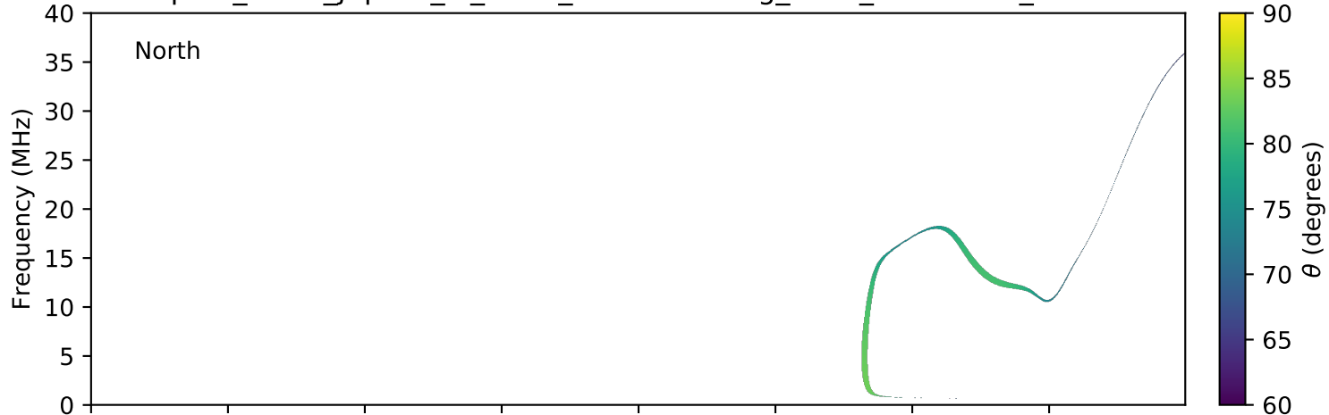
expres_earth_jupiter_io_isaac_lossc-wid1deg_3kev_20061231_v01.cdf
