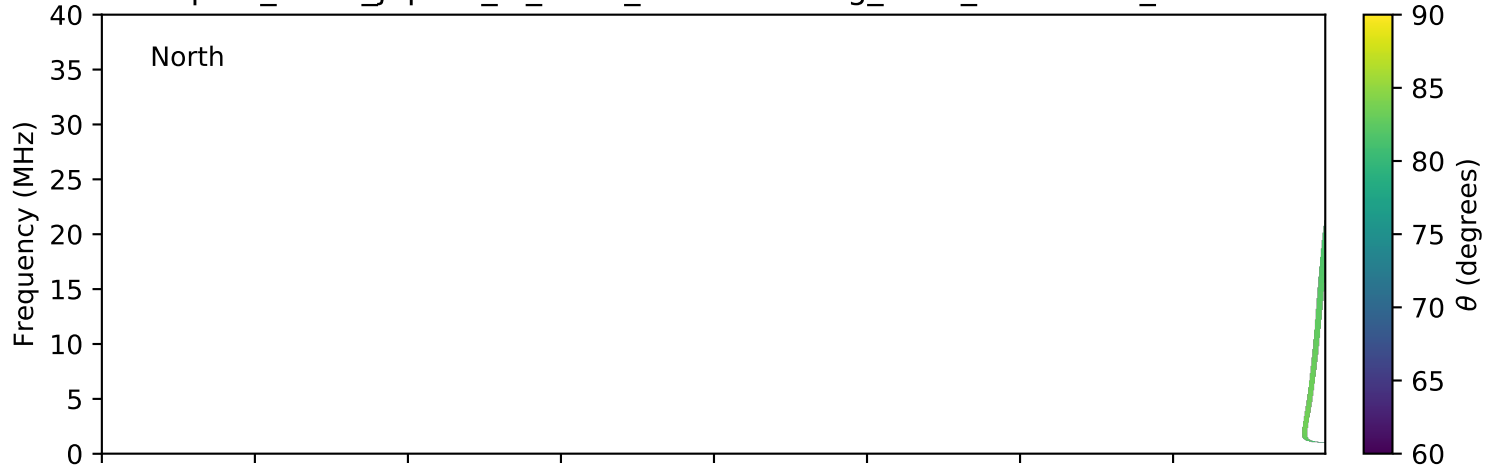
expres_earth_jupiter_io_isaac_lossc-wid1deg_3kev_20061229_v01.cdf
