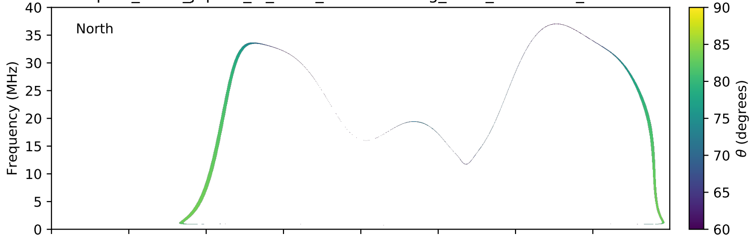
expres_earth_jupiter_io_isaac_lossc-wid1deg_3kev_20061228_v01.cdf
