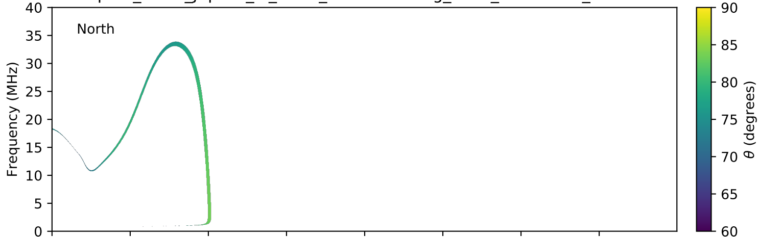
expres_earth_jupiter_io_isaac_lossc-wid1deg_3kev_20061227_v01.cdf
