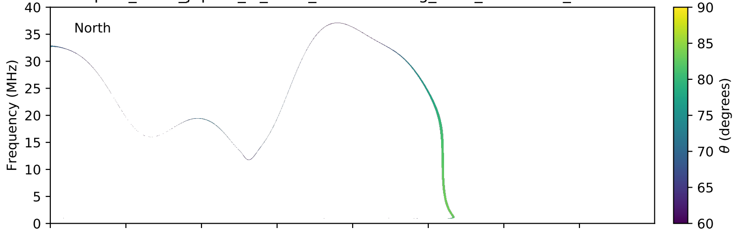
expres_earth_jupiter_io_isaac_lossc-wid1deg_3kev_20061223_v01.cdf
