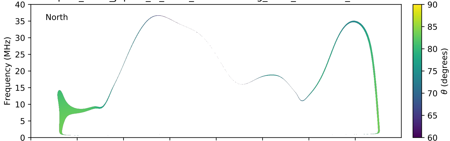
expres_earth_jupiter_io_isaac_lossc-wid1deg_3kev_20061221_v01.cdf
