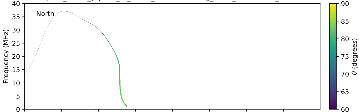
expres_earth_jupiter_io_isaac_lossc-wid1deg_3kev_20061218_v01.cdf
