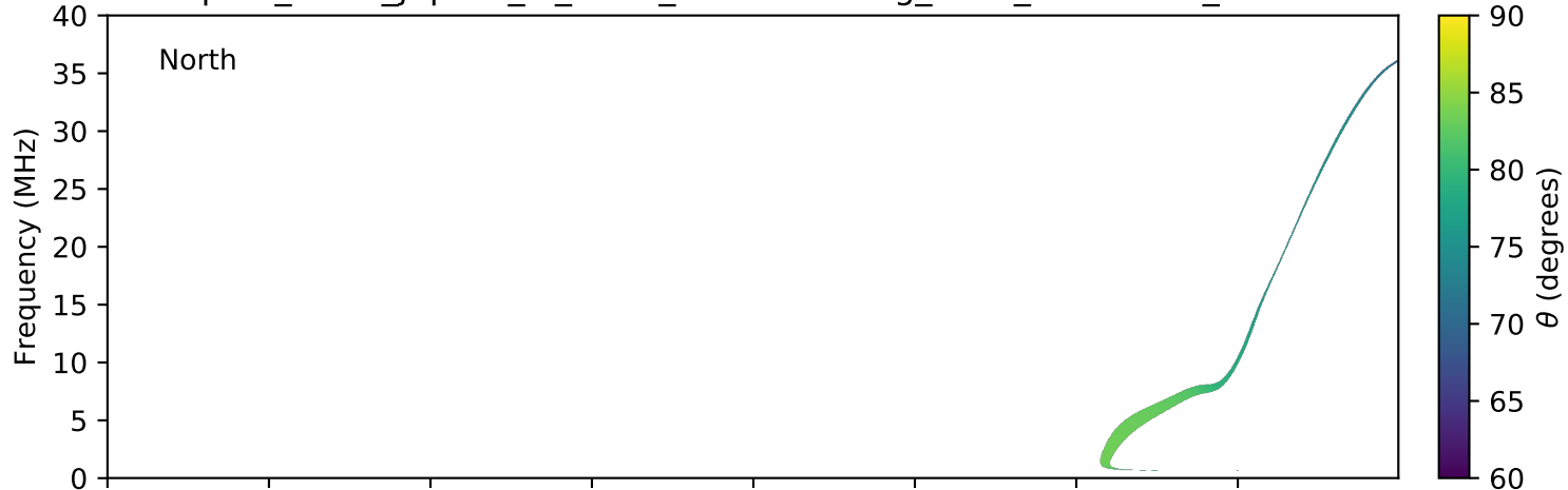
expres_earth_jupiter_io_isaac_lossc-wid1deg_3kev_20061215_v01.cdf
