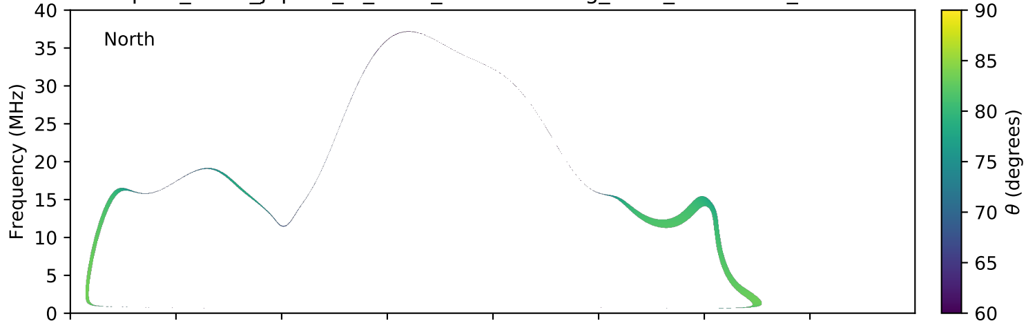
expres_earth_jupiter_io_isaac_lossc-wid1deg_3kev_20061214_v01.cdf
