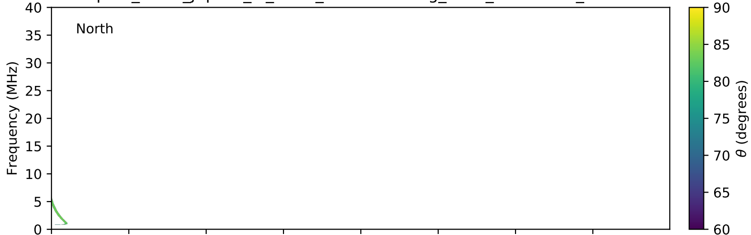
expres_earth_jupiter_io_isaac_lossc-wid1deg_3kev_20061213_v01.cdf
