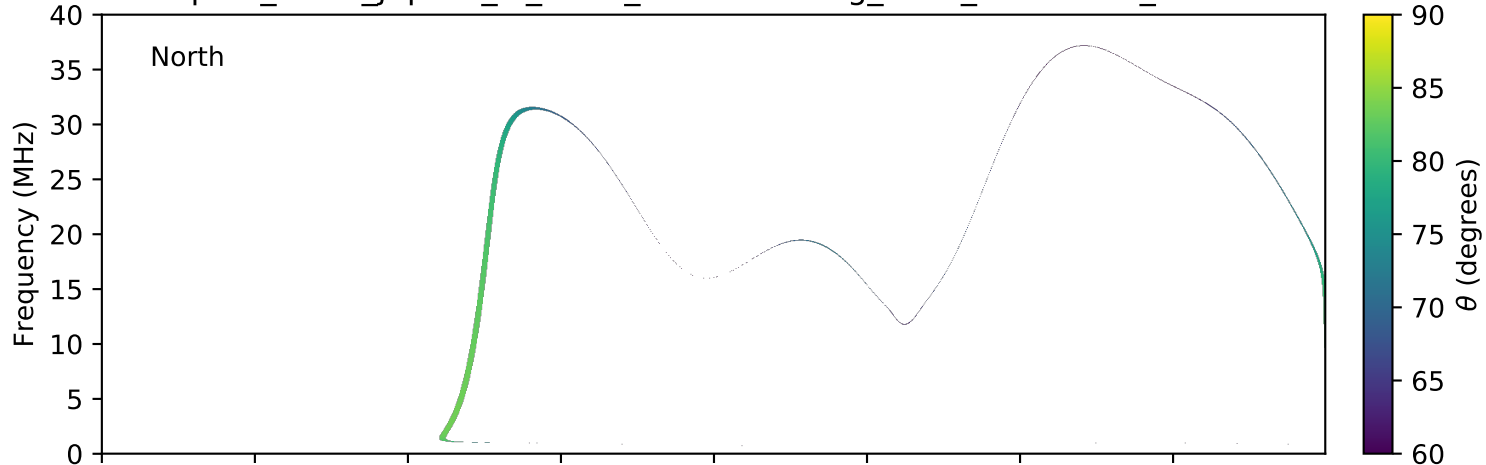
expres_earth_jupiter_io_isaac_lossc-wid1deg_3kev_20061212_v01.cdf
