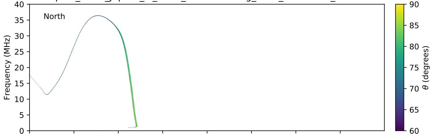
expres_earth_jupiter_io_isaac_lossc-wid1deg_3kev_20061211_v01.cdf
