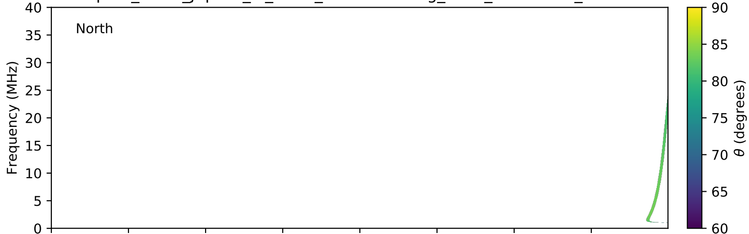
expres_earth_jupiter_io_isaac_lossc-wid1deg_3kev_20061206_v01.cdf
