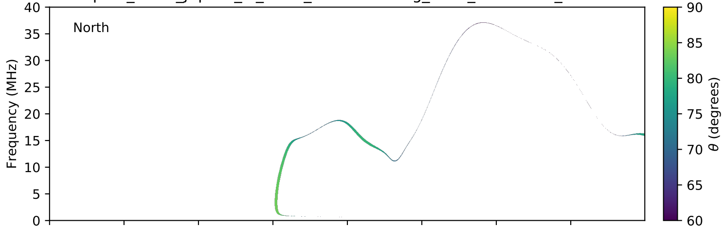
expres_earth_jupiter_io_isaac_lossc-wid1deg_3kev_20061203_v01.cdf
