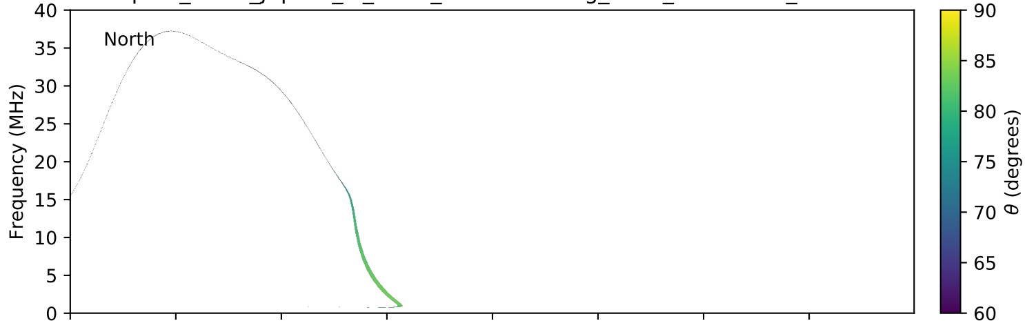
expres_earth_jupiter_io_isaac_lossc-wid1deg_3kev_20061202_v01.cdf
