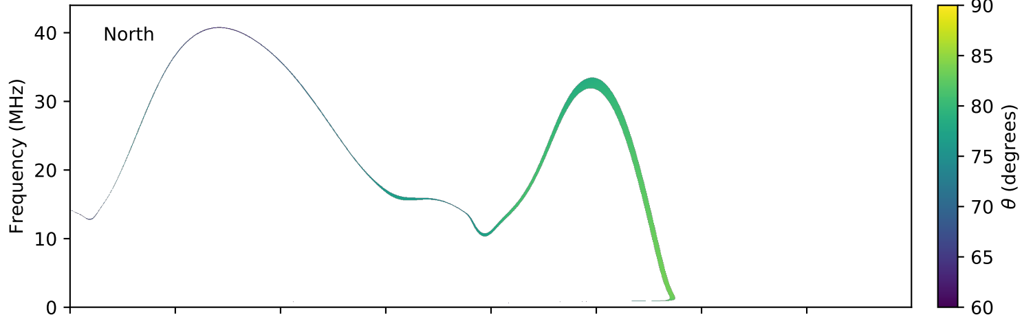
expres_earth_jupiter_europa_jrm09_lossc-wid1deg_3kev_20061231_v01.cdf
