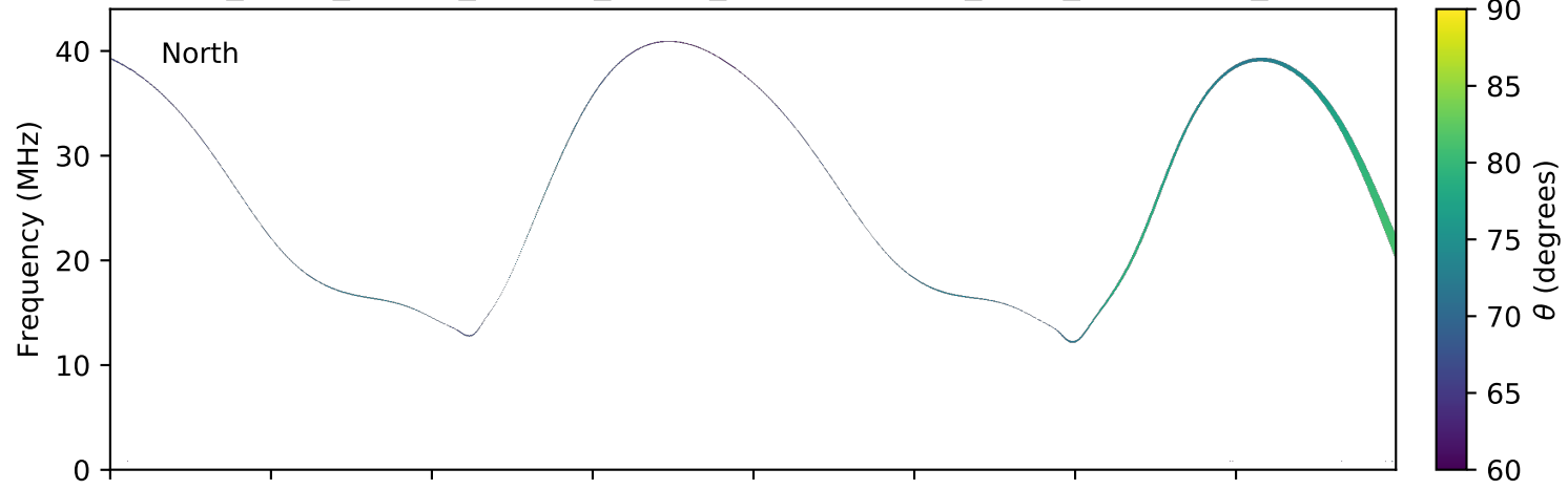
expres_earth_jupiter_europa_jrm09_lossc-wid1deg_3kev_20061227_v01.cdf
