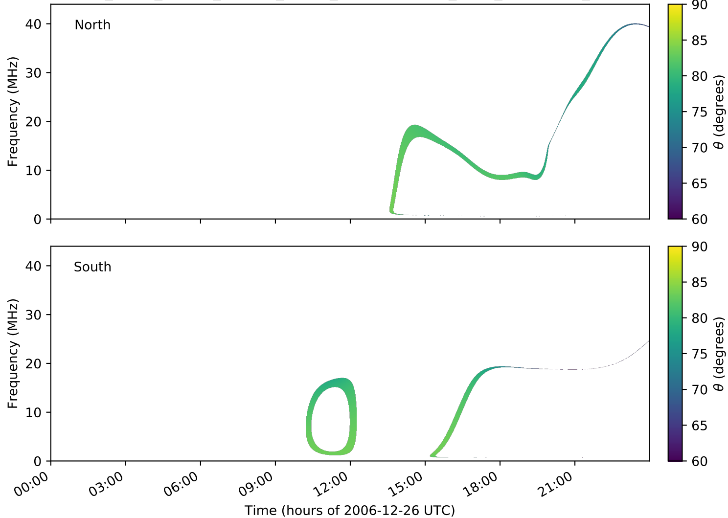
expres_earth_jupiter_europa_jrm09_lossc-wid1deg_3kev_20061226_v01.cdf
