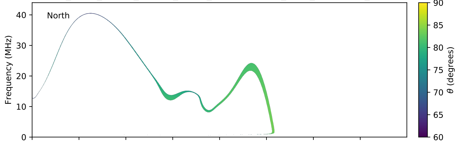
expres_earth_jupiter_europa_jrm09_lossc-wid1deg_3kev_20061224_v01.cdf
