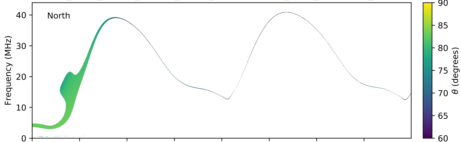
expres_earth_jupiter_europa_jrm09_lossc-wid1deg_3kev_20061216_v01.cdf
