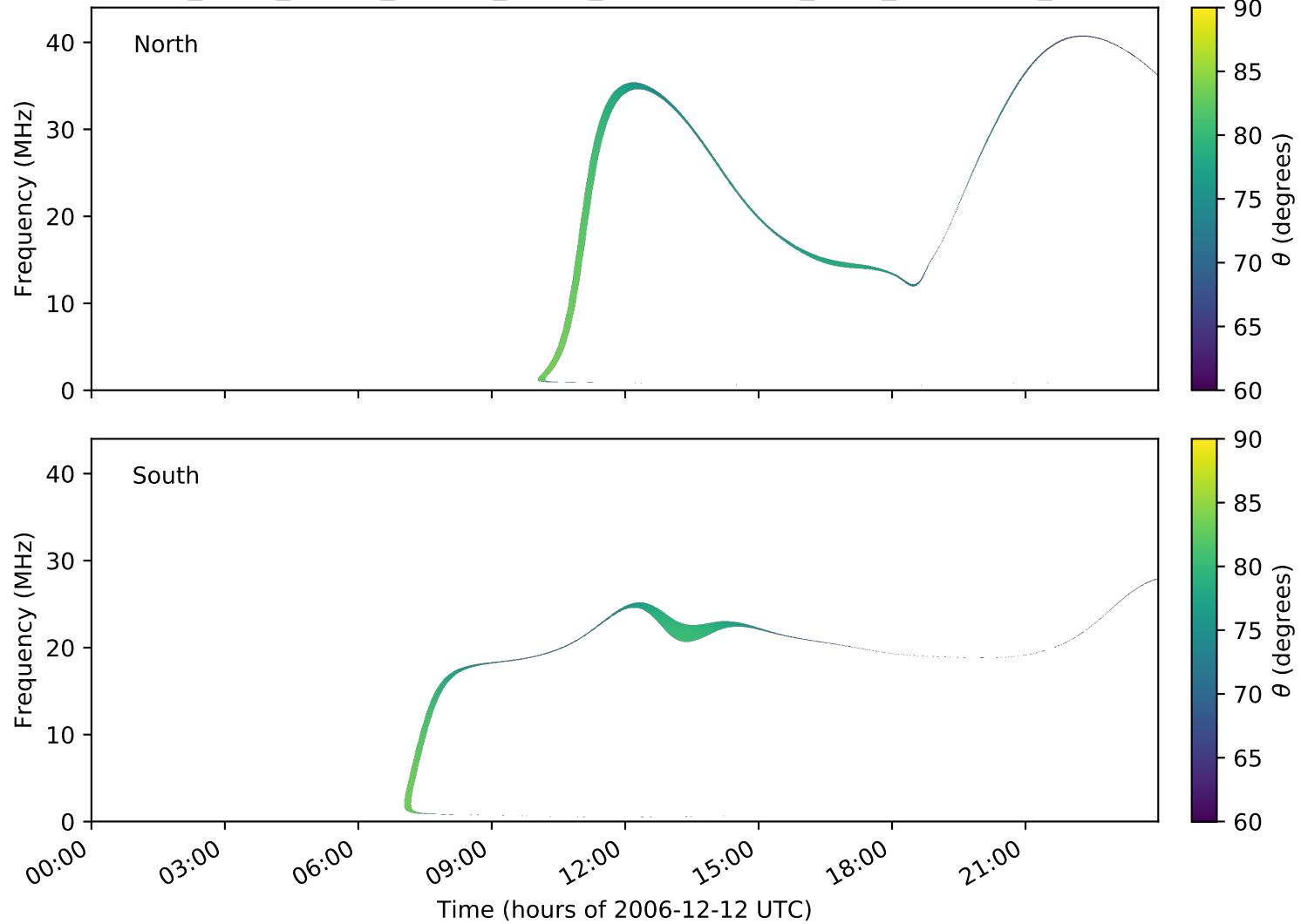
expres_earth_jupiter_europa_jrm09_lossc-wid1deg_3kev_20061212_v01.cdf
