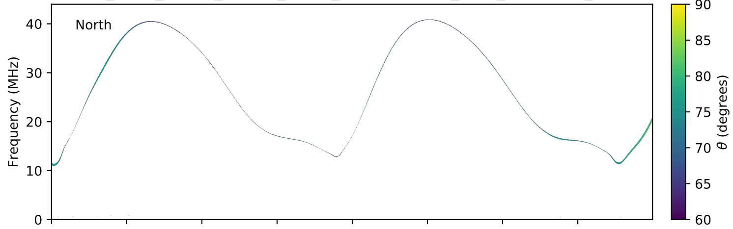
expres_earth_jupiter_europa_jrm09_lossc-wid1deg_3kev_20061202_v01.cdf
