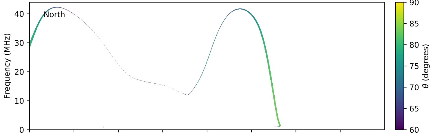
expres_earth_jupiter_io_jrm09_lossc-wid1deg_3kev_20061130_v01.cdf
