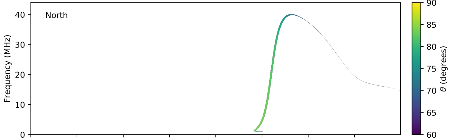
expres_earth_jupiter_io_jrm09_lossc-wid1deg_3kev_20061124_v01.cdf
