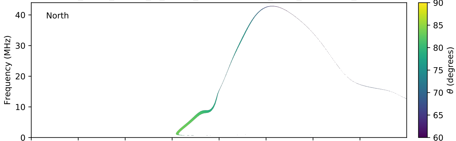
expres_earth_jupiter_io_jrm09_lossc-wid1deg_3kev_20061110_v01.cdf
