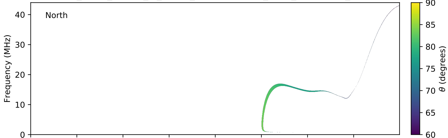
expres_earth_jupiter_io_jrm09_lossc-wid1deg_3kev_20061108_v01.cdf
