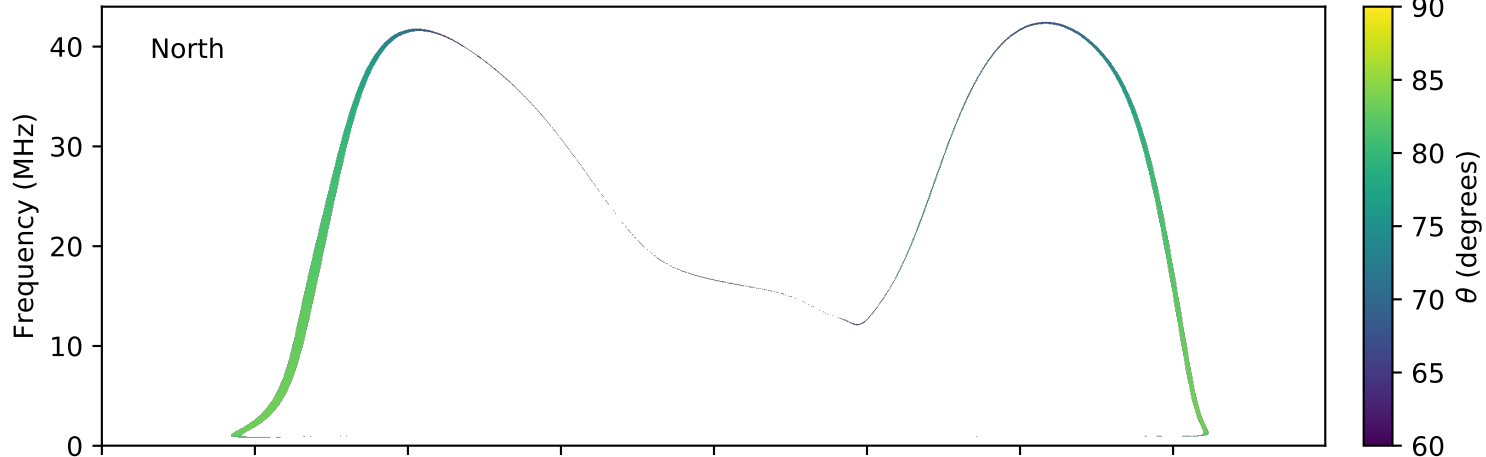
expres_earth_jupiter_io_jrm09_lossc-wid1deg_3kev_20061105_v01.cdf
