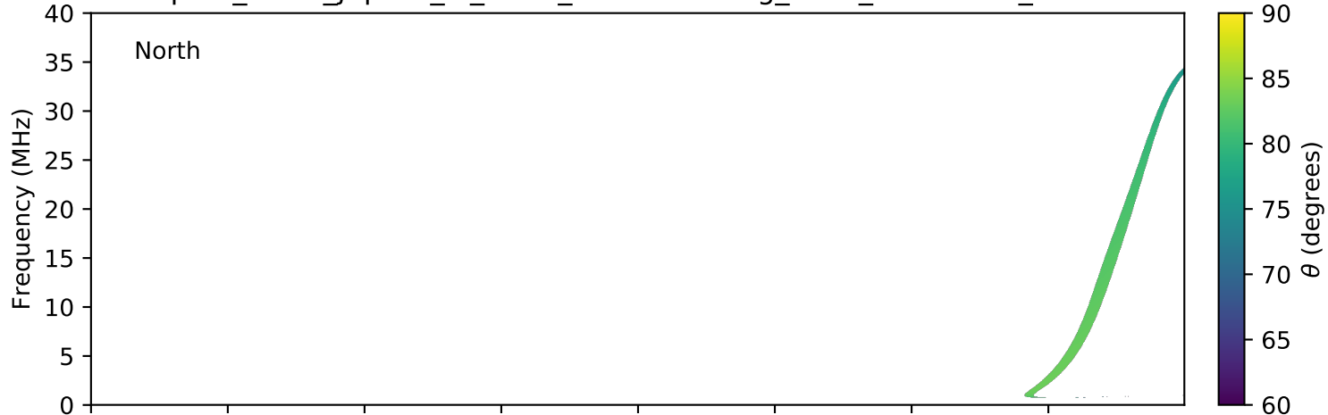
expres_earth_jupiter_io_isaac_lossc-wid1deg_3kev_20061129_v01.cdf
