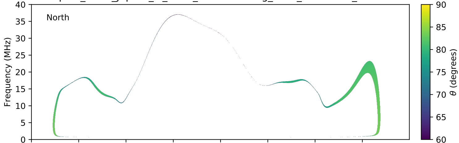
expres_earth_jupiter_io_isaac_lossc-wid1deg_3kev_20061128_v01.cdf
