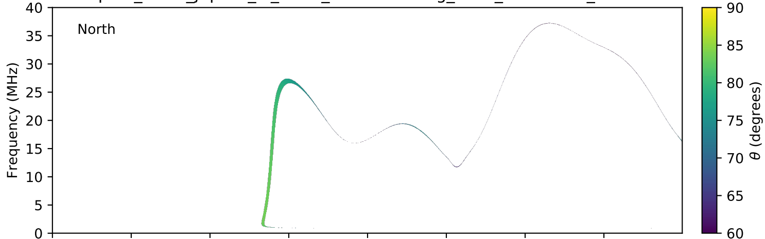
expres_earth_jupiter_io_isaac_lossc-wid1deg_3kev_20061126_v01.cdf
