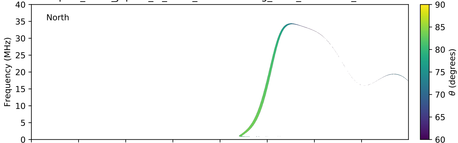
expres_earth_jupiter_io_isaac_lossc-wid1deg_3kev_20061124_v01.cdf
