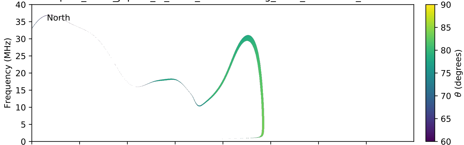
expres_earth_jupiter_io_isaac_lossc-wid1deg_3kev_20061123_v01.cdf
