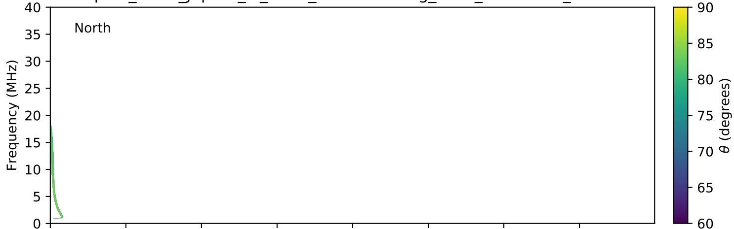
expres_earth_jupiter_io_isaac_lossc-wid1deg_3kev_20061120_v01.cdf
