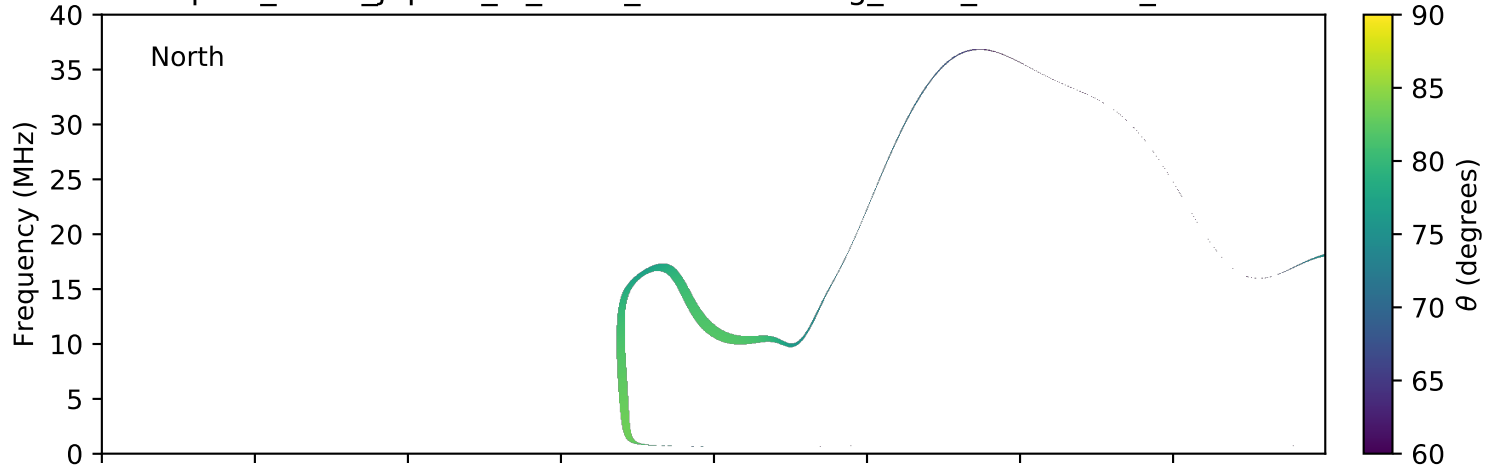
expres_earth_jupiter_io_isaac_lossc-wid1deg_3kev_20061117_v01.cdf
