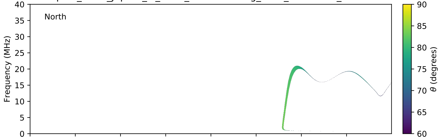
expres_earth_jupiter_io_isaac_lossc-wid1deg_3kev_20061115_v01.cdf
