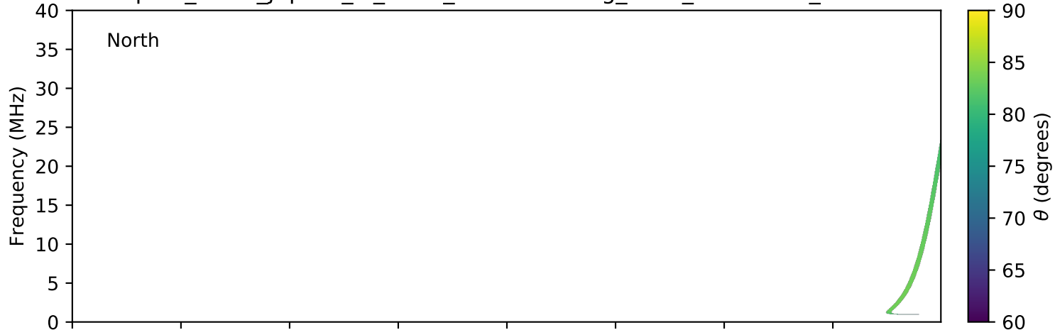
expres_earth_jupiter_io_isaac_lossc-wid1deg_3kev_20061113_v01.cdf
