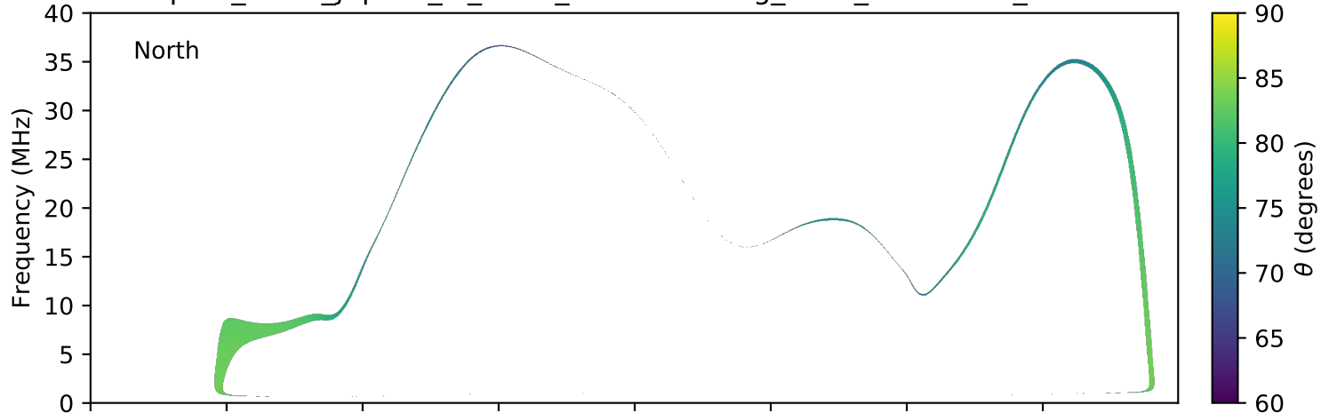
expres_earth_jupiter_io_isaac_lossc-wid1deg_3kev_20061112_v01.cdf
