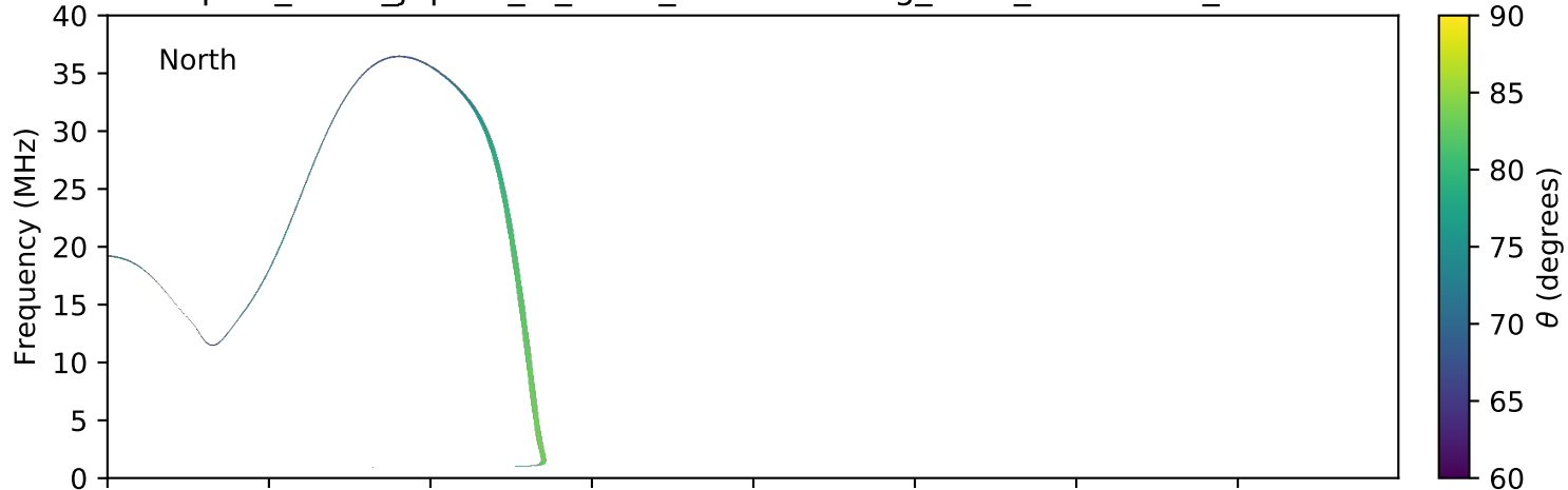
expres_earth_jupiter_io_isaac_lossc-wid1deg_3kev_20061102_v01.cdf
