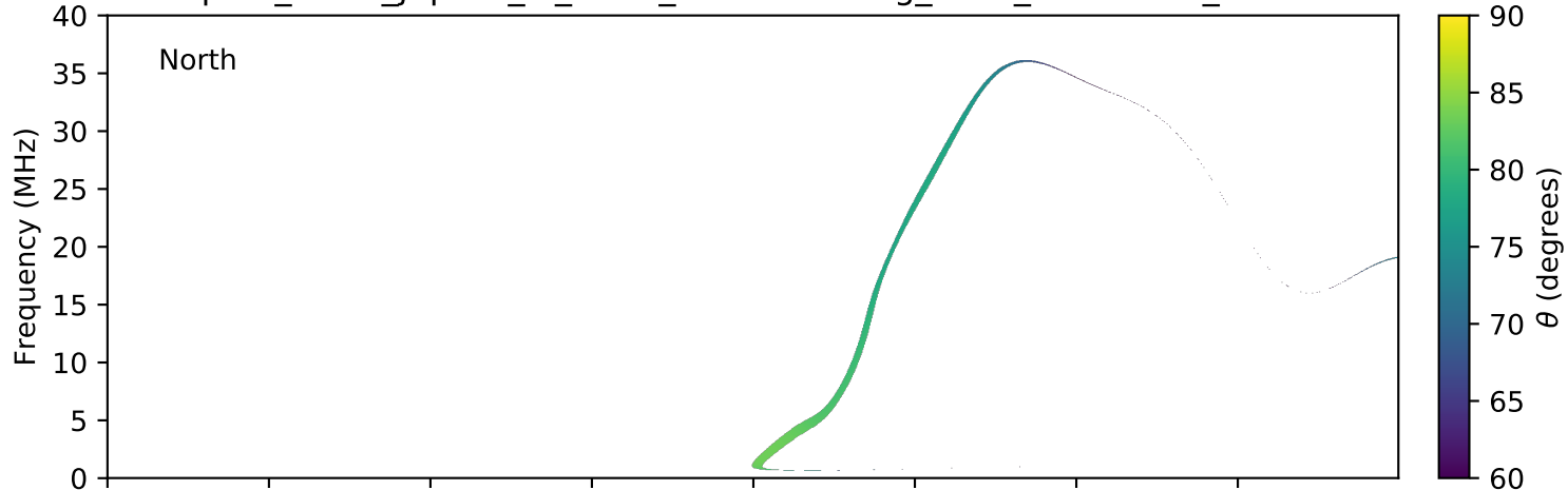
expres_earth_jupiter_io_isaac_lossc-wid1deg_3kev_20061101_v01.cdf
