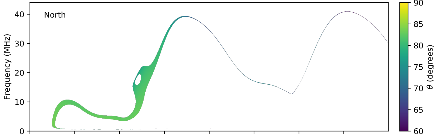
expres_earth_jupiter_europa_jrm09_lossc-wid1deg_3kev_20061128_v01.cdf
