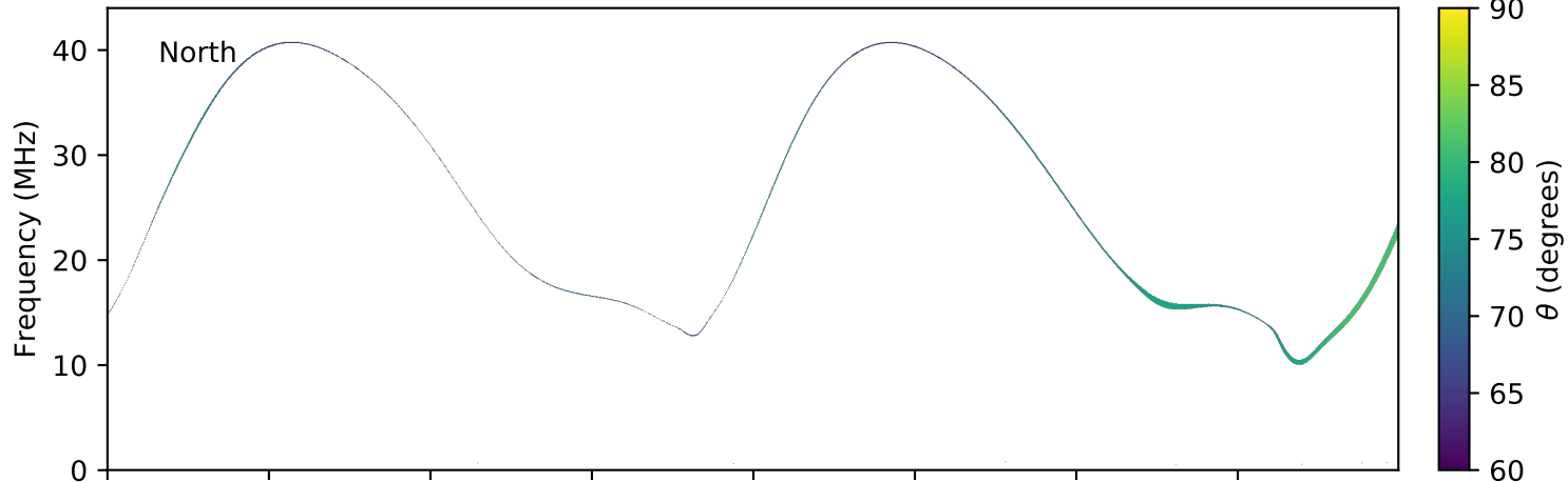
expres_earth_jupiter_europa_jrm09_lossc-wid1deg_3kev_20061125_v01.cdf
