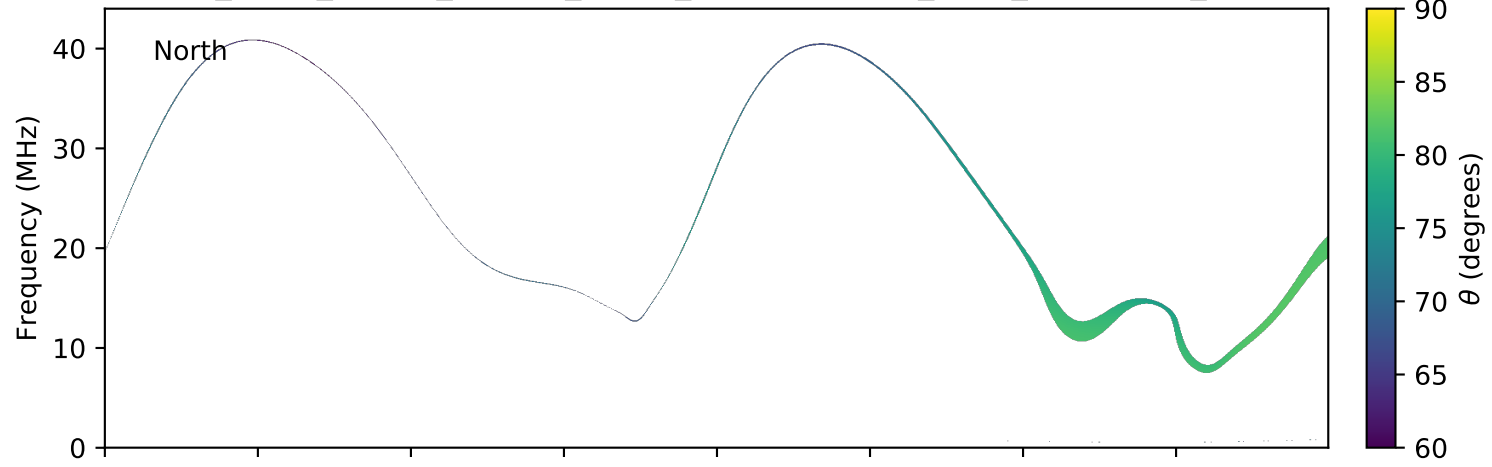
expres_earth_jupiter_europa_jrm09_lossc-wid1deg_3kev_20061118_v01.cdf
