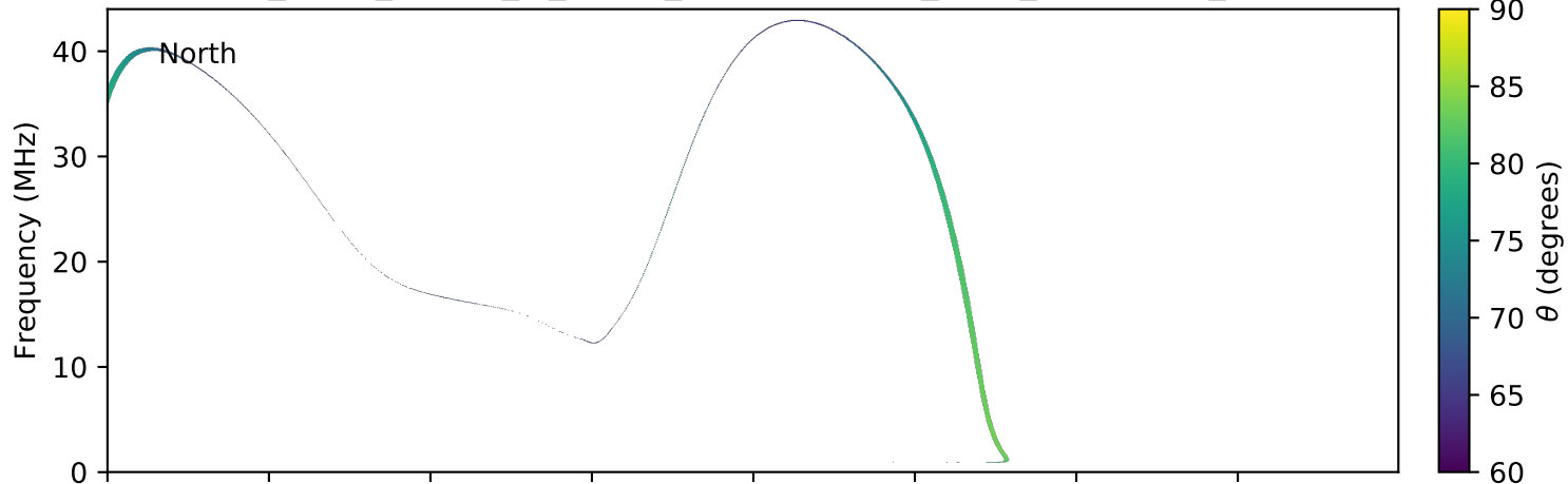
expres_earth_jupiter_io_jrm09_lossc-wid1deg_3kev_20060929_v01.cdf
