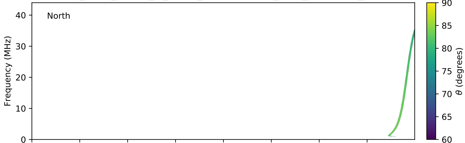
expres_earth_jupiter_io_jrm09_lossc-wid1deg_3kev_20060928_v01.cdf
