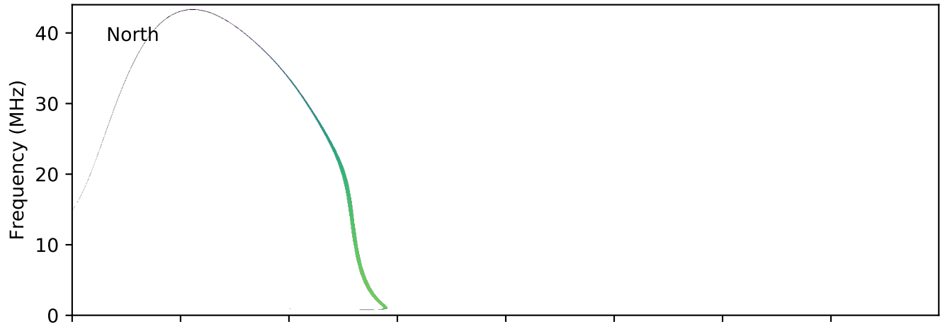
expres_earth_jupiter_io_jrm09_lossc-wid1deg_3kev_20060924_v01.cdf
