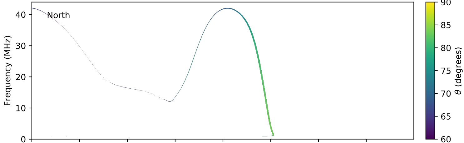
expres_earth_jupiter_io_jrm09_lossc-wid1deg_3kev_20060922_v01.cdf
